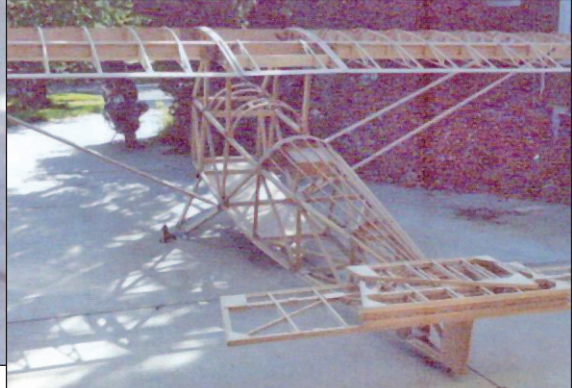
Waller's plane, modeled using plans from 1934, is nearing completion.
